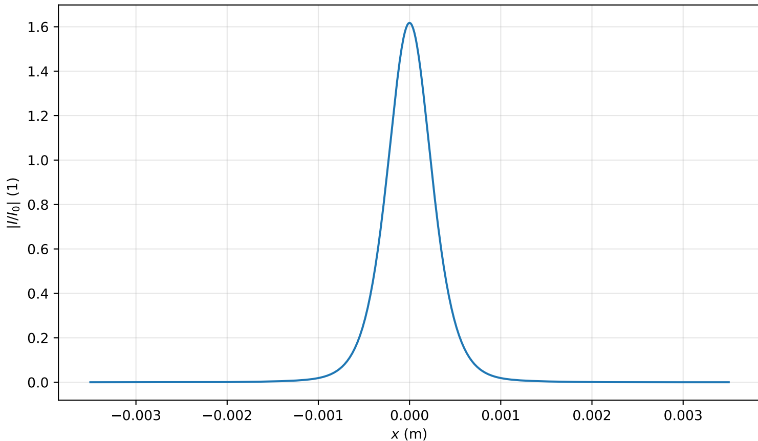
Intensity profile I(x, y = 0, z = 2.548m)/I_0 , P_{in}=0.9P_{cr} , artificial time
